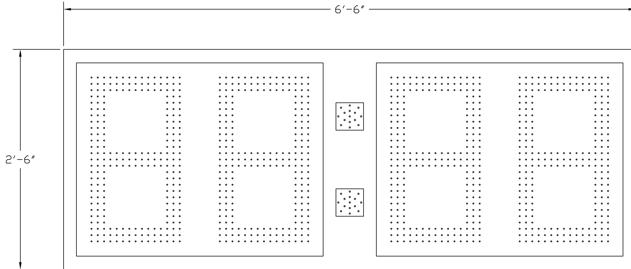
PT-063024-06-2 OUTDOOR 4-DIGIT PITCH TIMER USING 24"H AMBER LED DIGITS WITH AMBER LED LIT COLON
