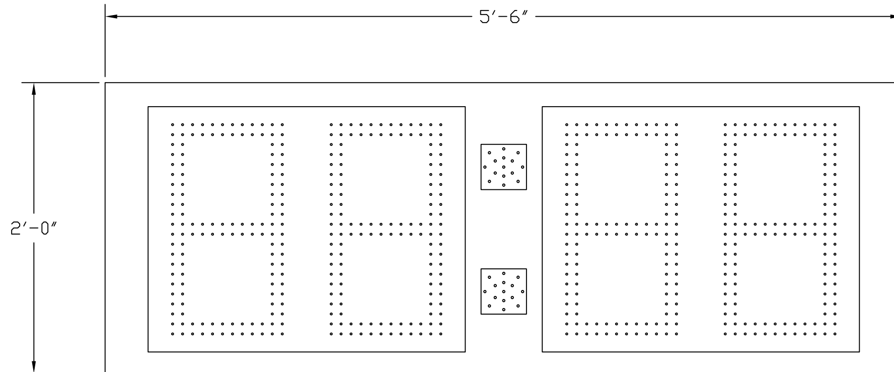
PT-052418-06-2 OUTDOOR 4-DIGIT PITCH TIMER USING 18"H AMBER LED DIGITS WITH AMBER LED LIT COLON
