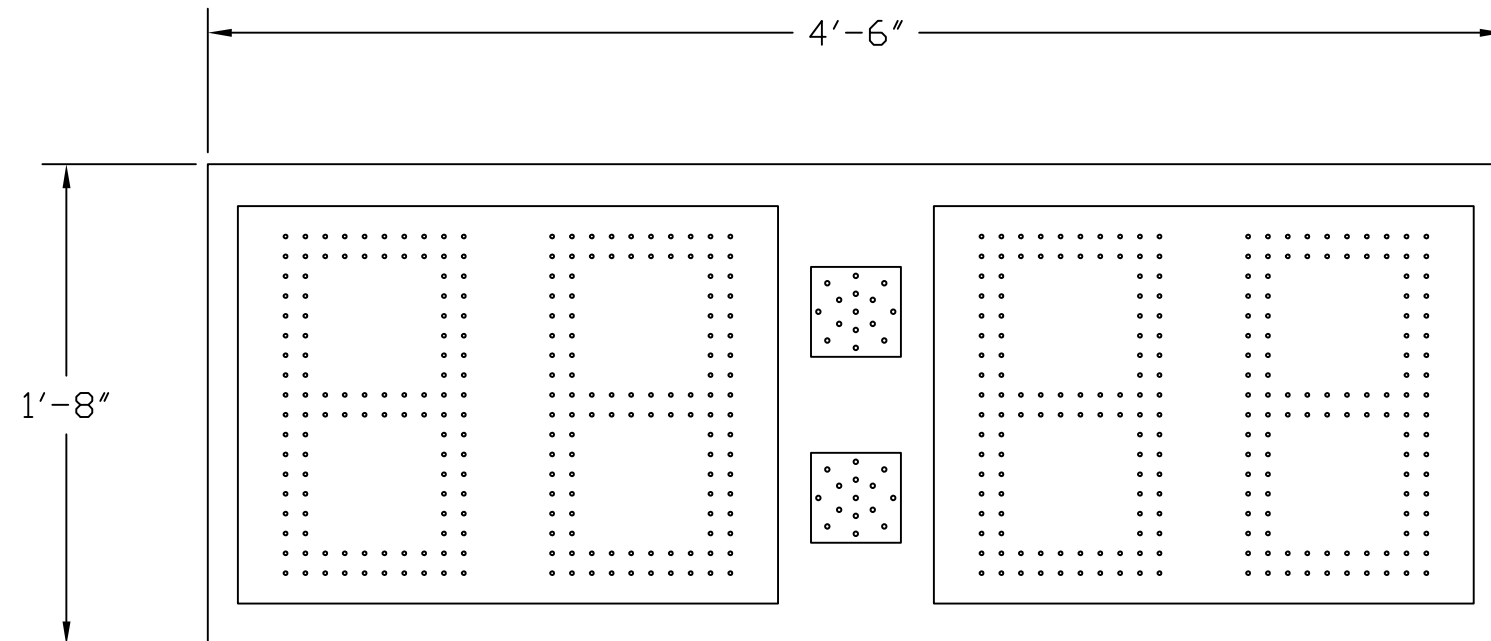
PT-042015-06-2 OUTDOOR 4-DIGIT PITCH TIMER USING 15"H AMBER LED DIGITS, AMBER LED LIT COLON
