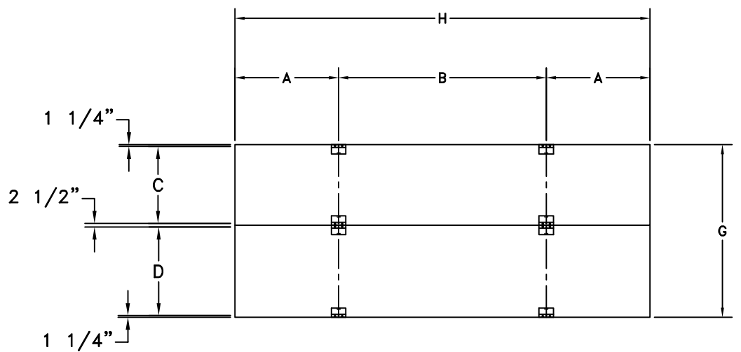
HANGER BRACKETS BACK VIEW
