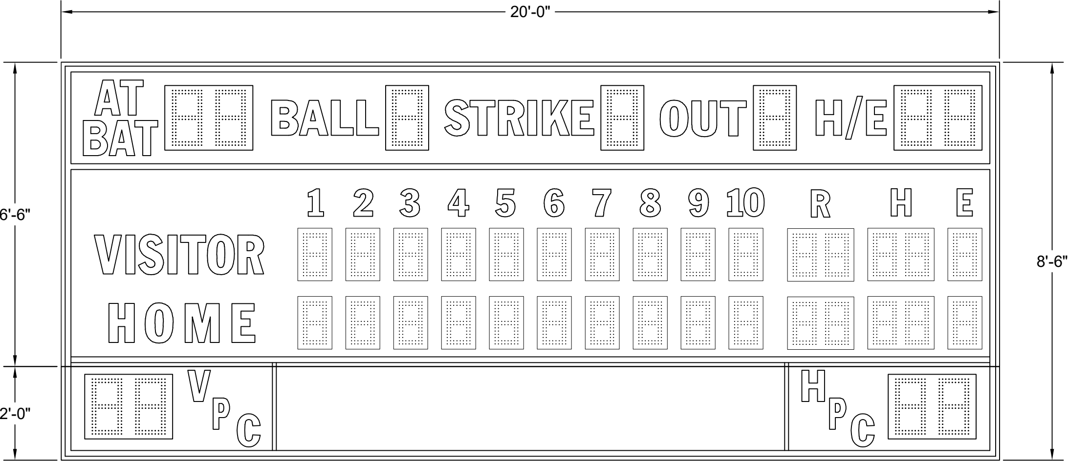
BA-7220PC-2 (15"H DIGITS MOVED TO ENDS OF PITCH COUNT SECTION, ADDED TRIM)
