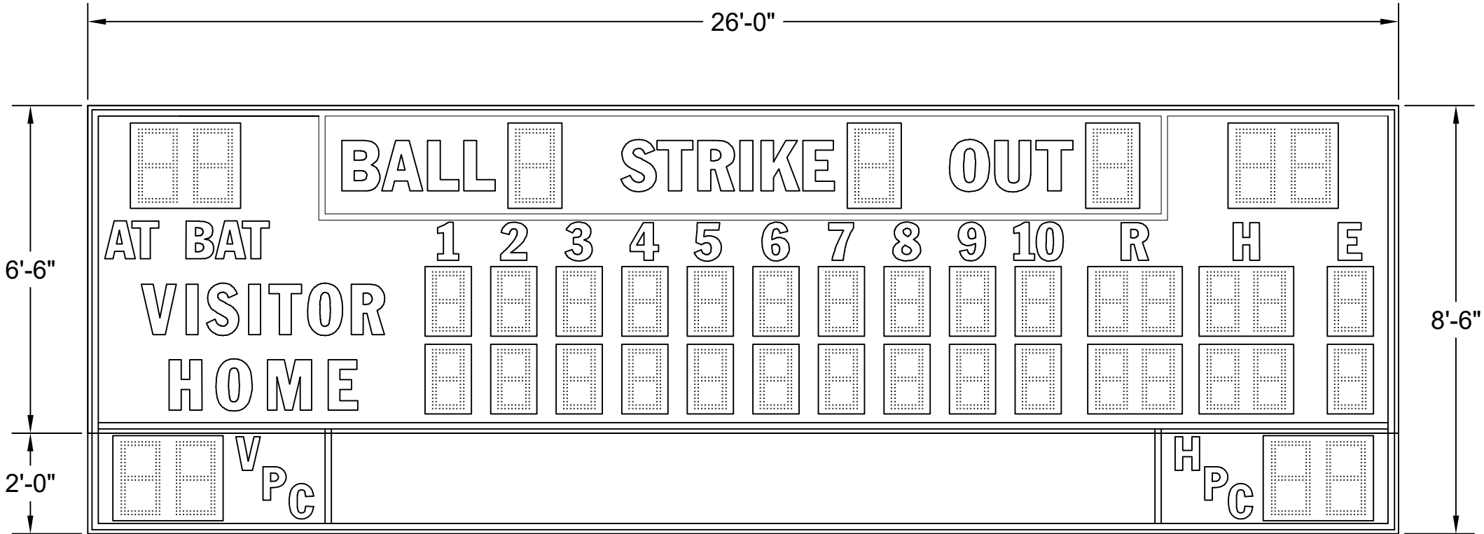
BA-7126PC-2 (18"H DIGITS MOVED TO THE ENDS OF PITCH COUNT SECTION, ADDED TRIM)
