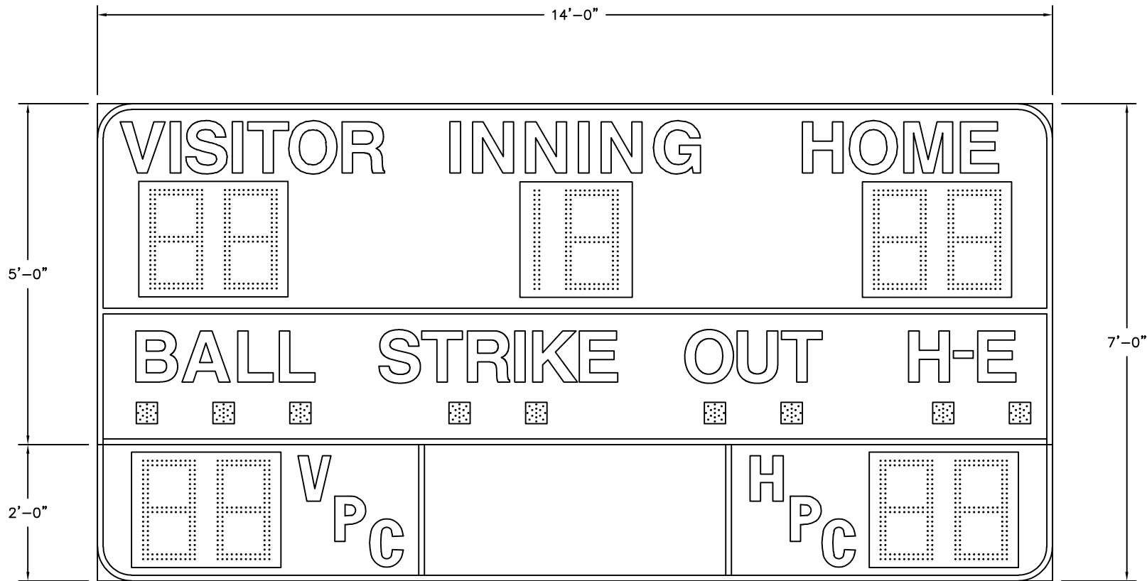
BA-7100PC-2 (18"H DIGITS MOVED TO ENDS OF PITCH COUNT SECTION, ADDED TRIM)
