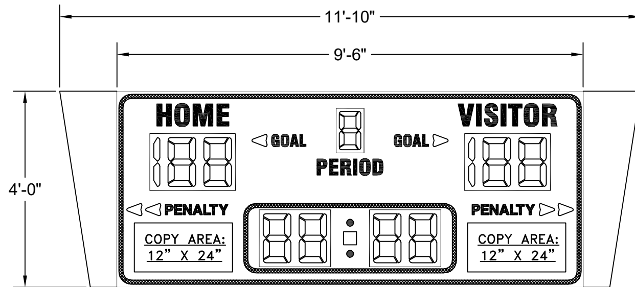
HK-1800-4 FOUR-SIDED HOCKEY SCOREBOARD SIDE 1 OF 4 SHOWN - ALL OTHERS TYPICAL
