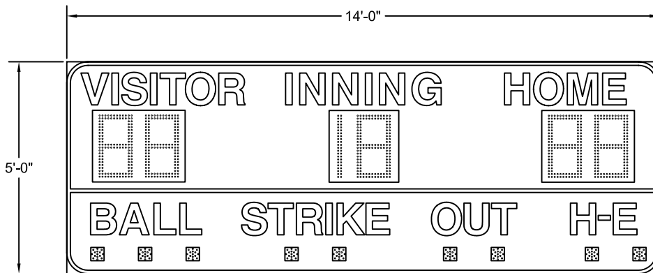
BA-7100-2 7'-0" L HANGER SPACING, STANDARD J BRACKETS
