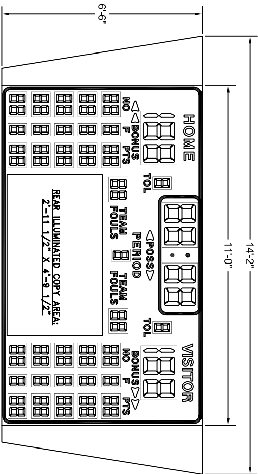
BB-1855B-4 FOUR-SIDED BASKETBALL SCOREBOARD SIDE 1 OF 4 SHOWN - ALL OTHERS TYPICAL
